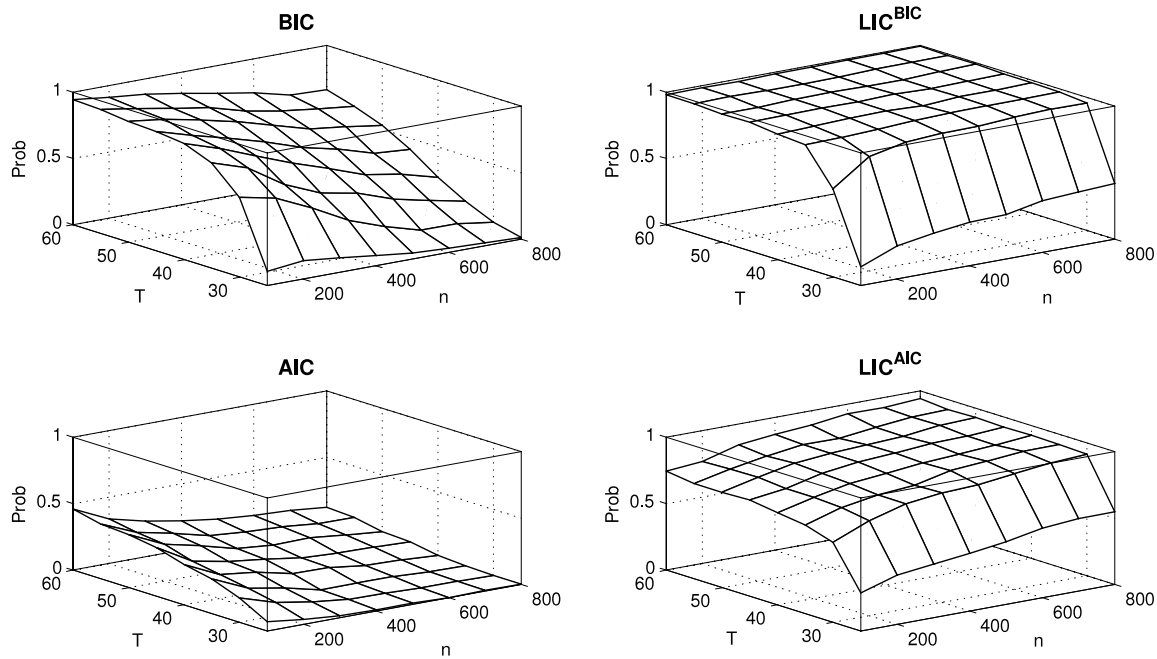
Fig. 1. Correct lag order selection frequencies when p_0 = 3 .
