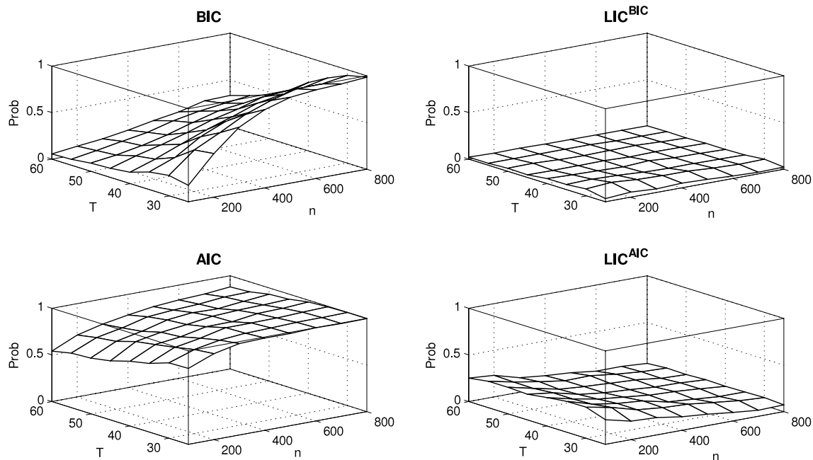
Fig. 2. Over selection frequencies when p_0 = 3 .
