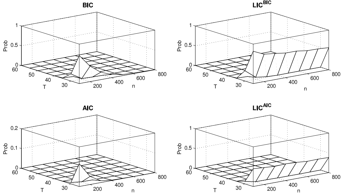
Fig. 3. Under selection frequencies when p_0 = 3 .
