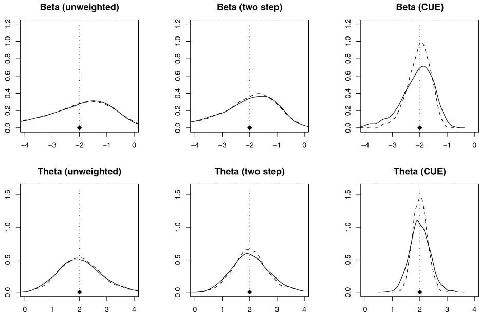
FIGURE 2.—Kernel densities. The upper panel plots are for \beta estimates and the lower panel plots for \theta are estimates. From left to right are shown unweighted GMM, usual two step GMM, and CUE estimation. The solid lines are for n = 50 and T = 40 ; the dashed lines are for n = 100 and T = 80 ; the solid diamonds signify the true parameters.
