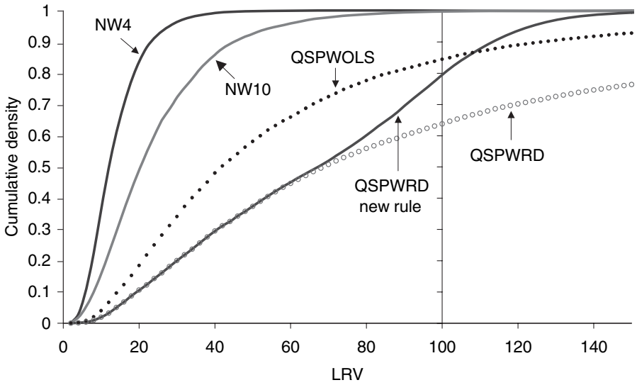
Figure 1. Empirical cumulative density function of various LRV estimators (true \Omega_t = 100 )
